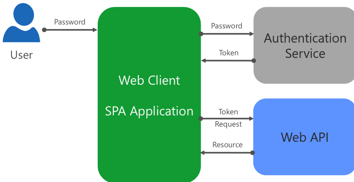
Figure 7-5. Token-based authentication for Web APIs.
